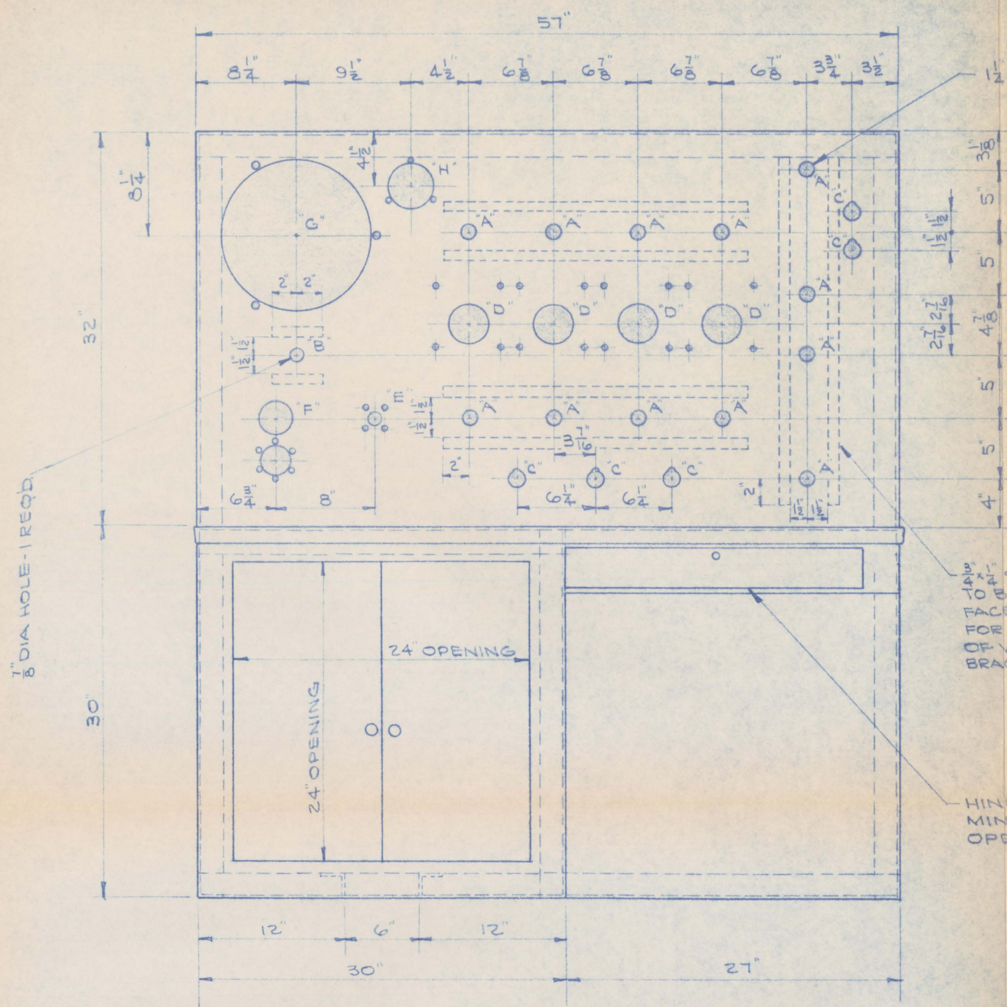
FRONT VIEW - CUTOUTS SCALE: 1 1/2" = 1'-0"
